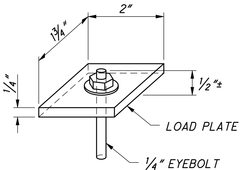
LOAD PLATE DETAIL
