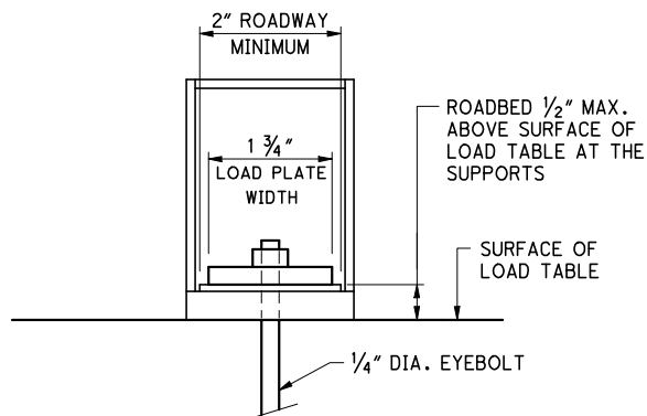
STRUCTURE SECTION
