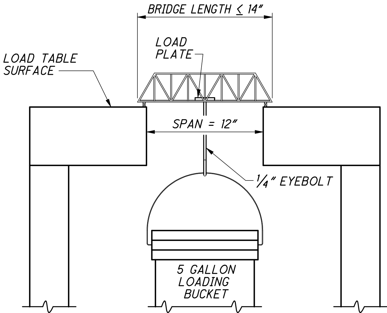
LOADING TABLE SETUP
